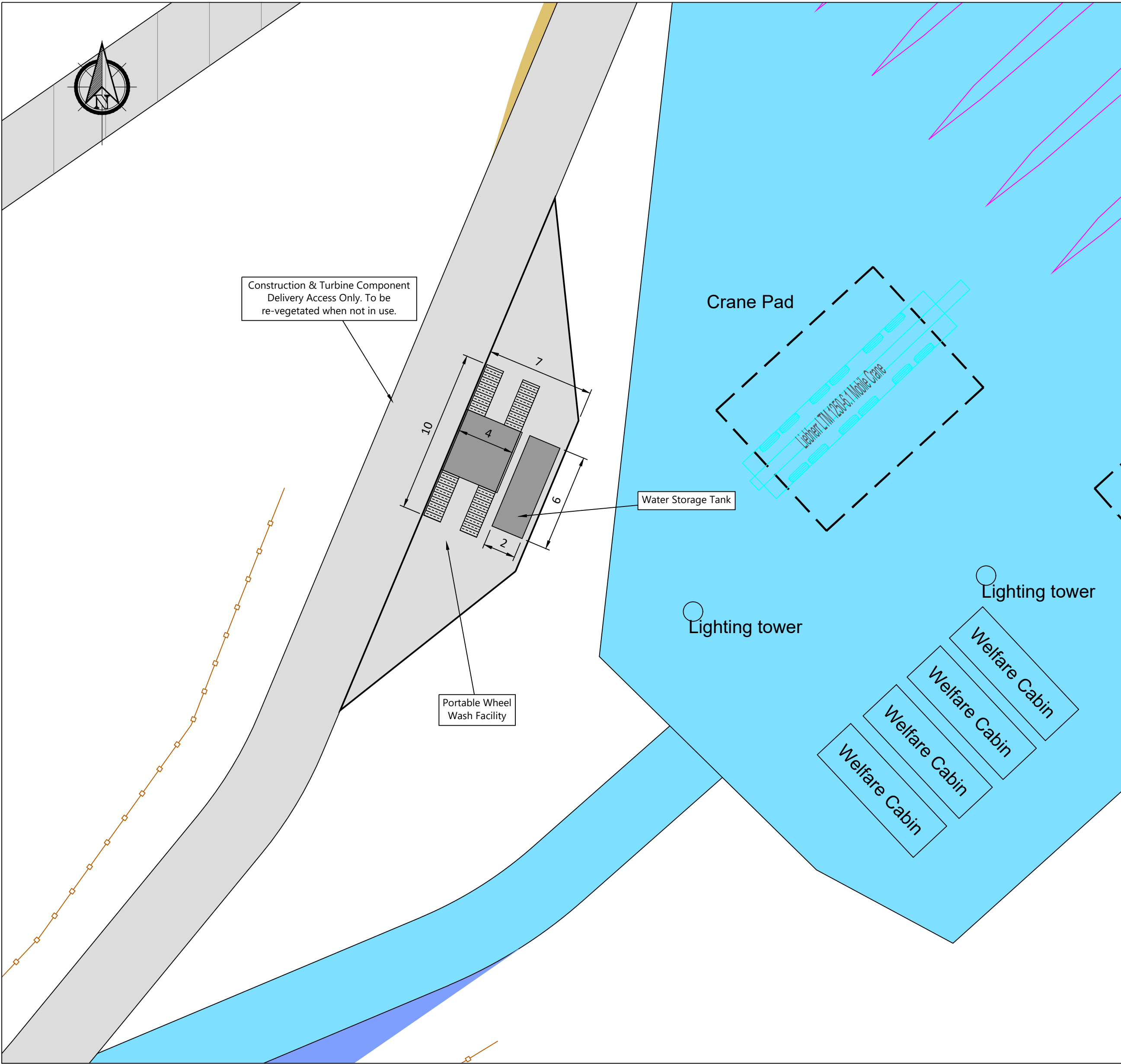
WHEEL WASH LAYOUT PLAN Scale 1:200
