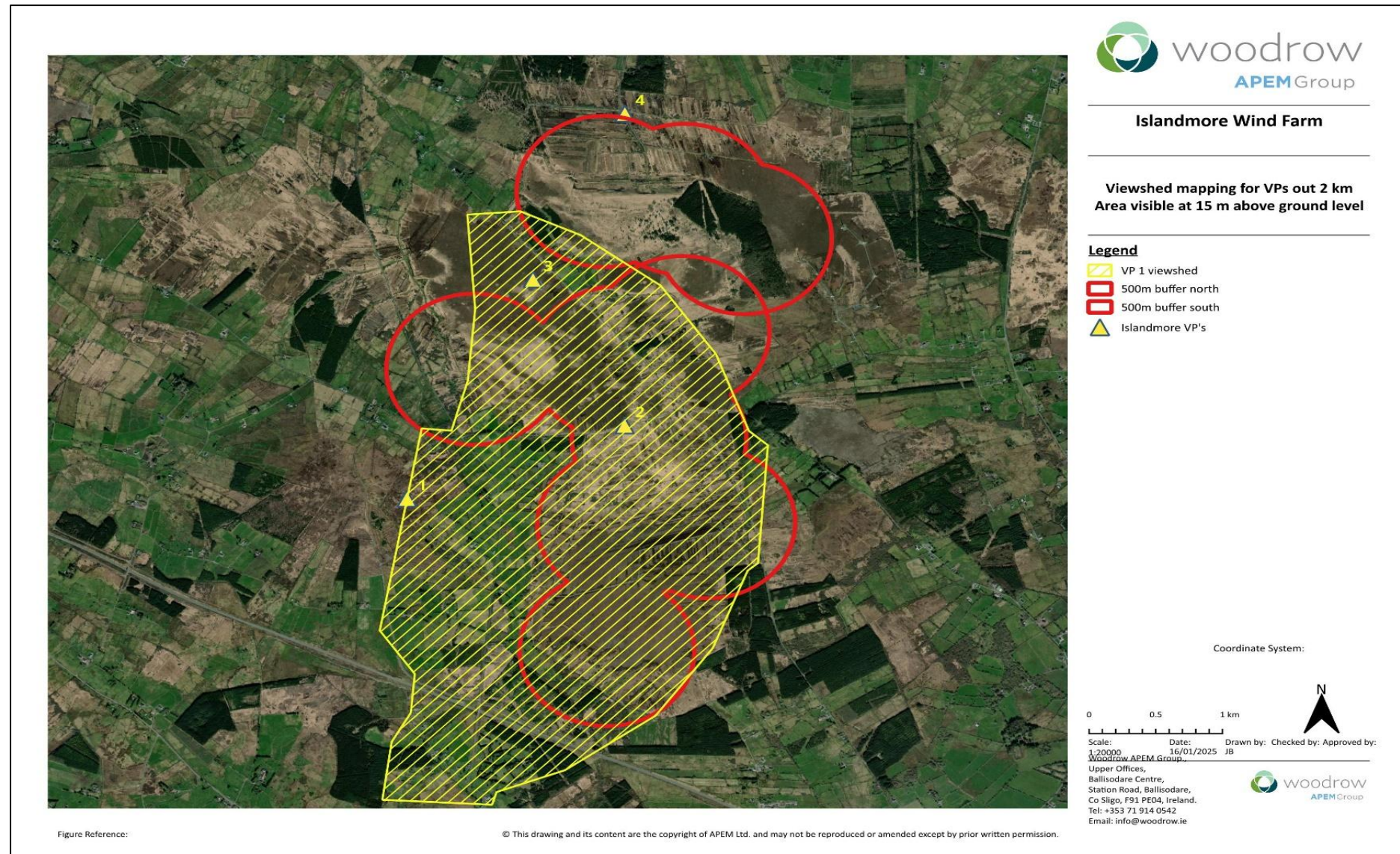
Figure 2: Viewshed for VP1 at 15 m above ground level and out to 2 km
